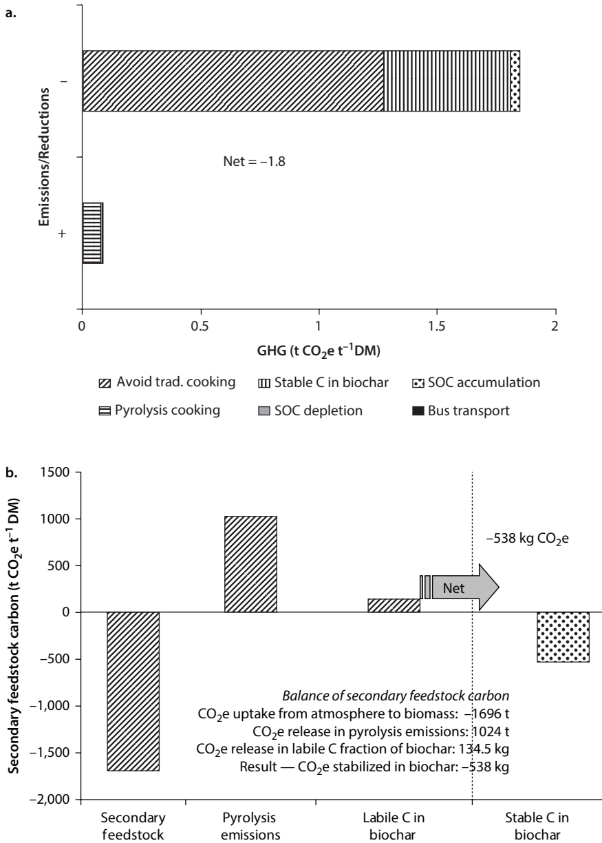
Figure 5.3 Sources of GHG Reductions and Emissions, and Carbon Balance for Secondary Feedstock
