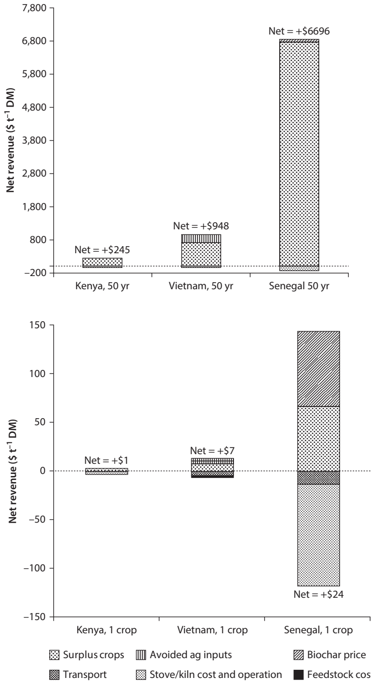
Figure 5.22 Comparison of Net Revenues of Three Case Studies: Kenya, Vietnam, and Senegal
