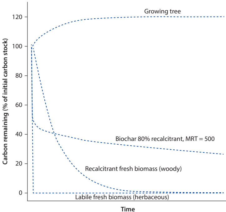
Figure 3.4 Alternative Scenarios for Biomass Carbon Dynamics
