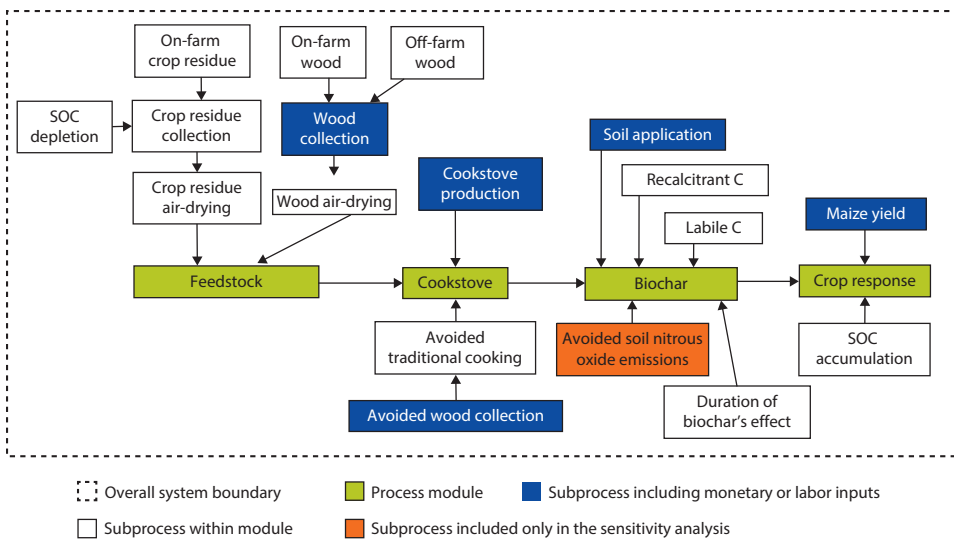
Figure 5.1 Schematic Flow Diagram for Biochar Production in a Pyrolysis Cookstove System
