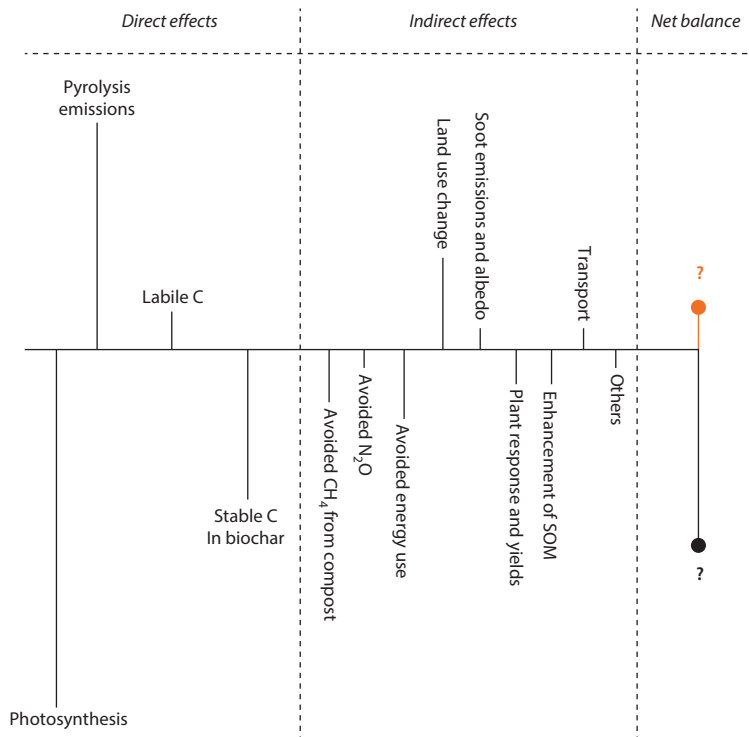
Figure 3.3 Impact of Biochar on Climate Change Mitigation
