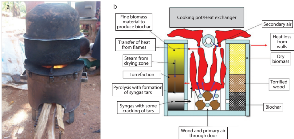
Figure 5.2 Pyrolysis Cookstove in Kenya Case Study
