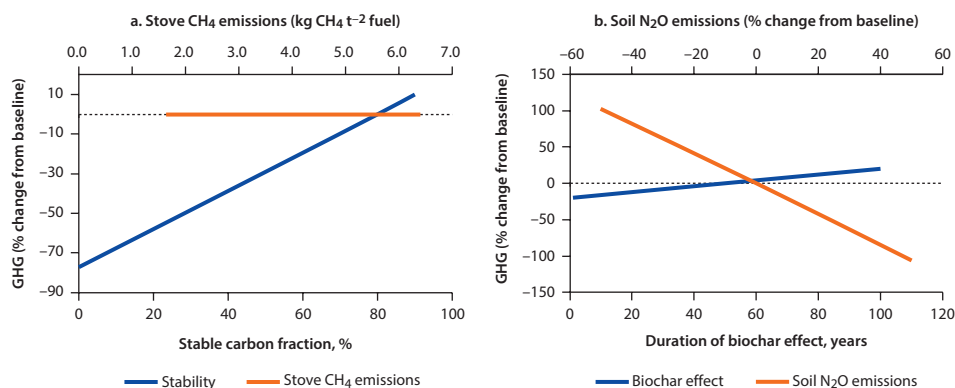
Figure 5.13 Sensitivity Analysis for Net GHG per Tonne of Dry Feedstock for Biochar System in Vietnam
