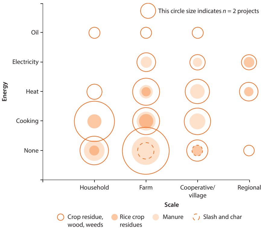
Figure 4.6 Typology of Biochar Systems by Type of Energy Recovery and Scale Showing Number of Projects with Each Type of Feedstock (n = 154)
