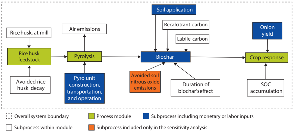
Figure 5.15 Schematic Flow Diagram for Rice Husk Biochar to Onion Production System in Senegal
