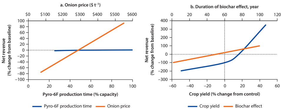
Figure 5.20 Sensitivity Analysis for Net Economic Balance per Tonne of Dry Feedstock for Biochar System in Senegal
