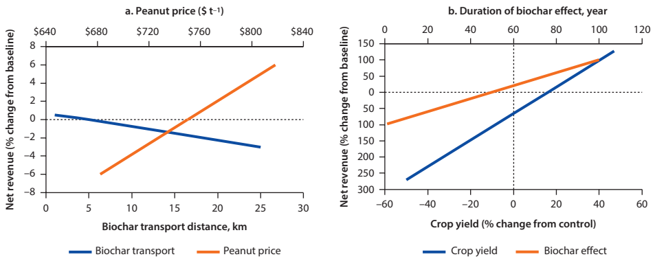
Figure 5.14 Sensitivity Analysis for Net Economic Balance per Tonne of Dry Feedstock for Biochar System in Vietnam
