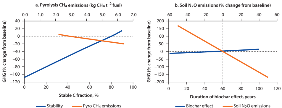
Figure 5.19 Sensitivity Analysis for Net GHG per Tonne of Dry Feedstock for Biochar System in Senegal
