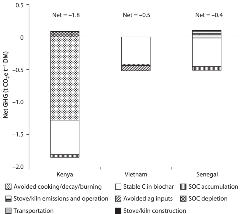
Figure 5.21 Comparison of Net GHG Balance of Three Case Studies: Kenya, Vietnam, and Senegal
