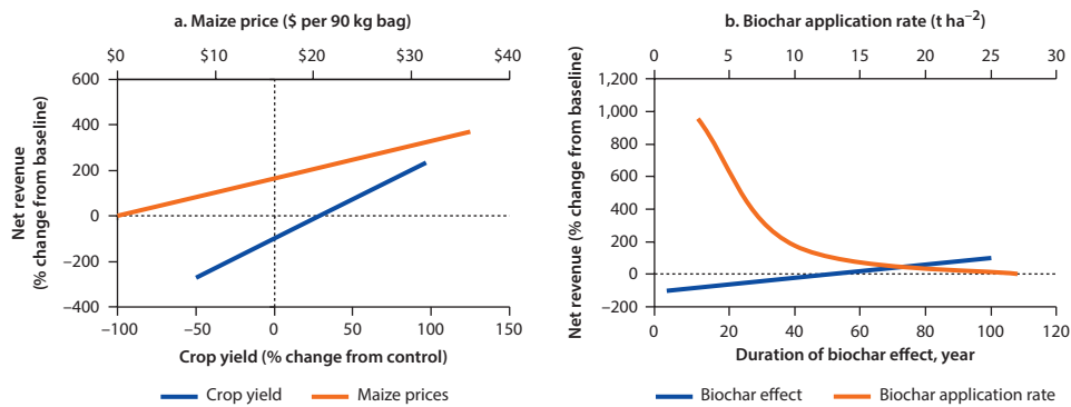
Figure 5.6 Sensitivity Analysis for Net Economic Balance per Tonne of Dry Secondary Feedstock for Pyrolysis Cookstove Biochar System in Kenya
