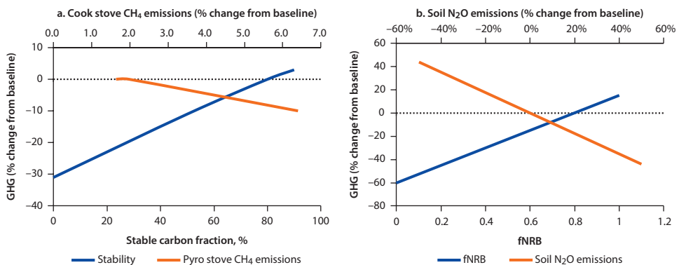
Figure 5.5 Sensitivity Analysis for Net GHG per Tonne of Dry Secondary Feedstock for Pyrolysis Cookstove Biochar System in Kenya
