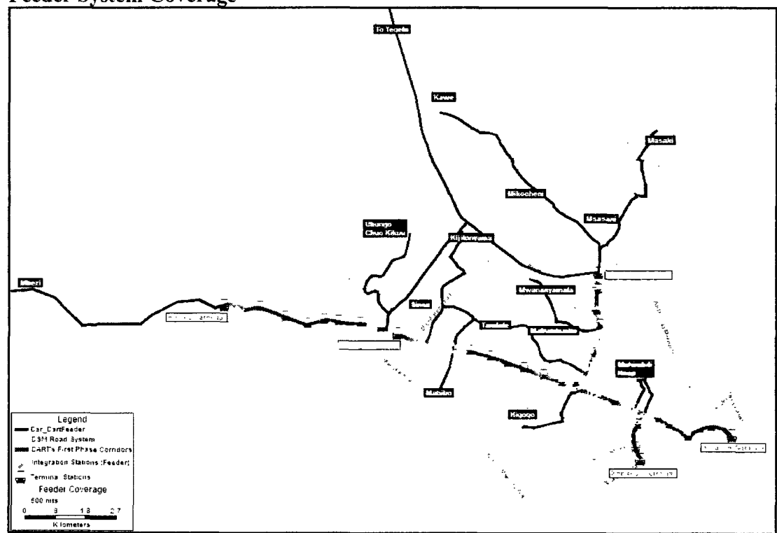
Figure 2.4.2.b Feeder System Coverage
