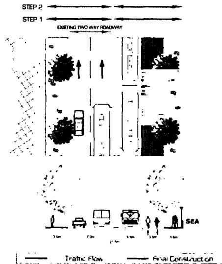
Figure 1.0.a Traffic Management on Kivukoni Front
