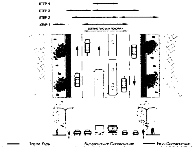
Figure 1.3.a Traffic Management – Morogoro Road – Bibi Titi to United Nations
