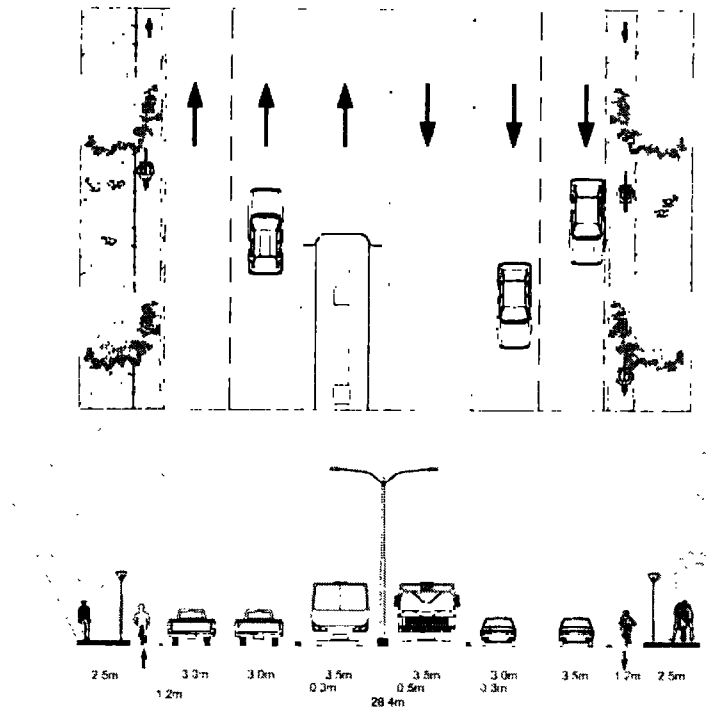
Figure 2.1.1.t Stretch 9 – Cross Section off Station
