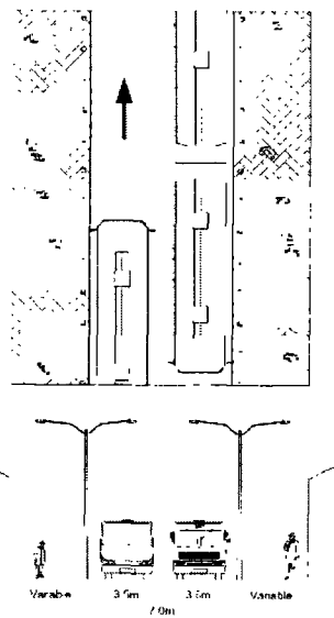
Figure 2.1.1.f Stretch 2 Cross Section off Station
