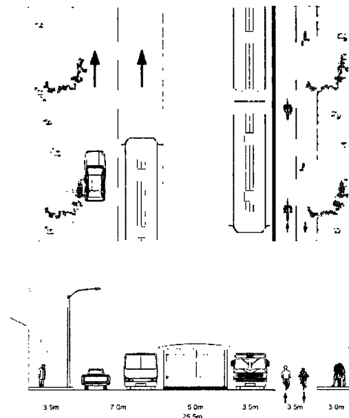
Figure 2.1.1.c Stretch 1 Cross Section at Station
