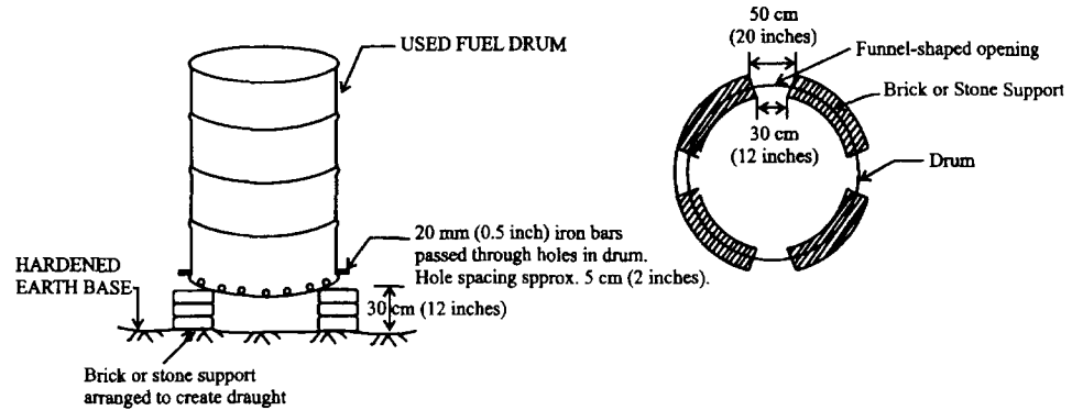
Figure 8-2. Stationary Incinerator
