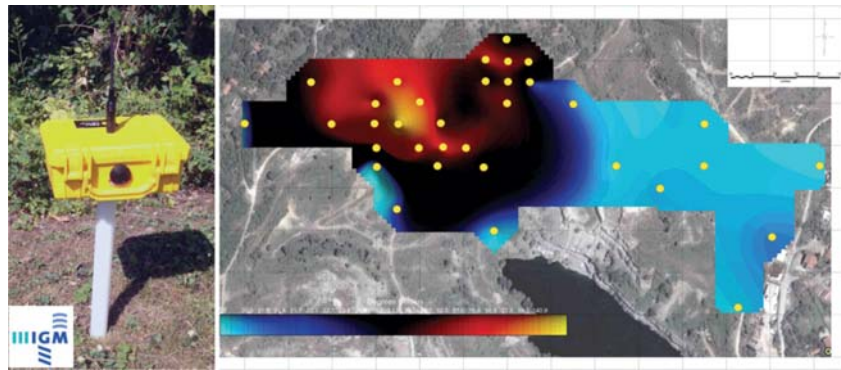
Figure 4.45. Left: Equipment deployed for monitoring ground temperature at 2-meter depth Right: Relative ground temperature gridded and displayed over an air photo of a survey area.
