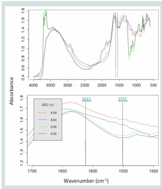
Figure 1 — Example of soil spectral signatures of four samples from the Ethiopia LASER study with different levels of soil organic carbon.
