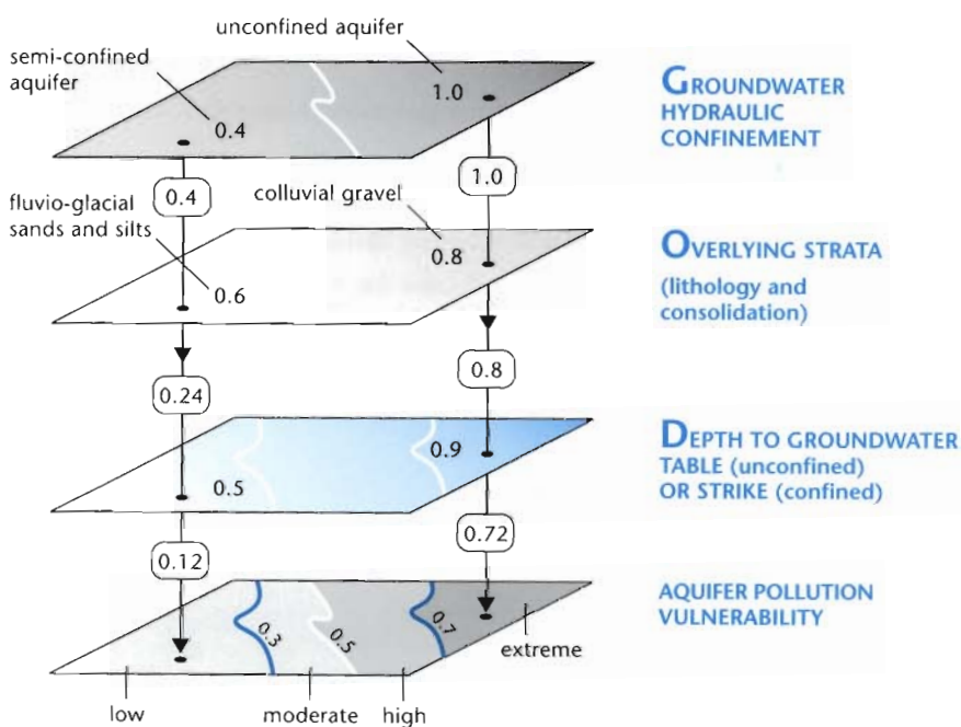
Figure 1.5 Generation of aquifer pollution vulnerability map using the GOD system
