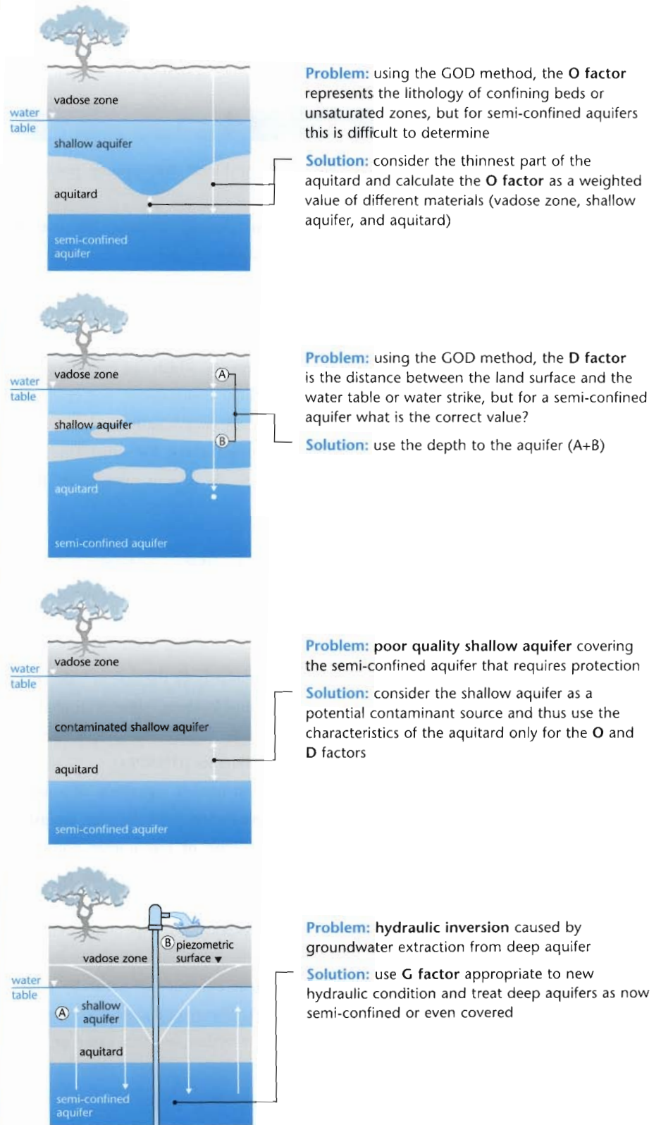
Figure 1.4 Interpretation of the pollution vulnerability of semi-confined aquifers
