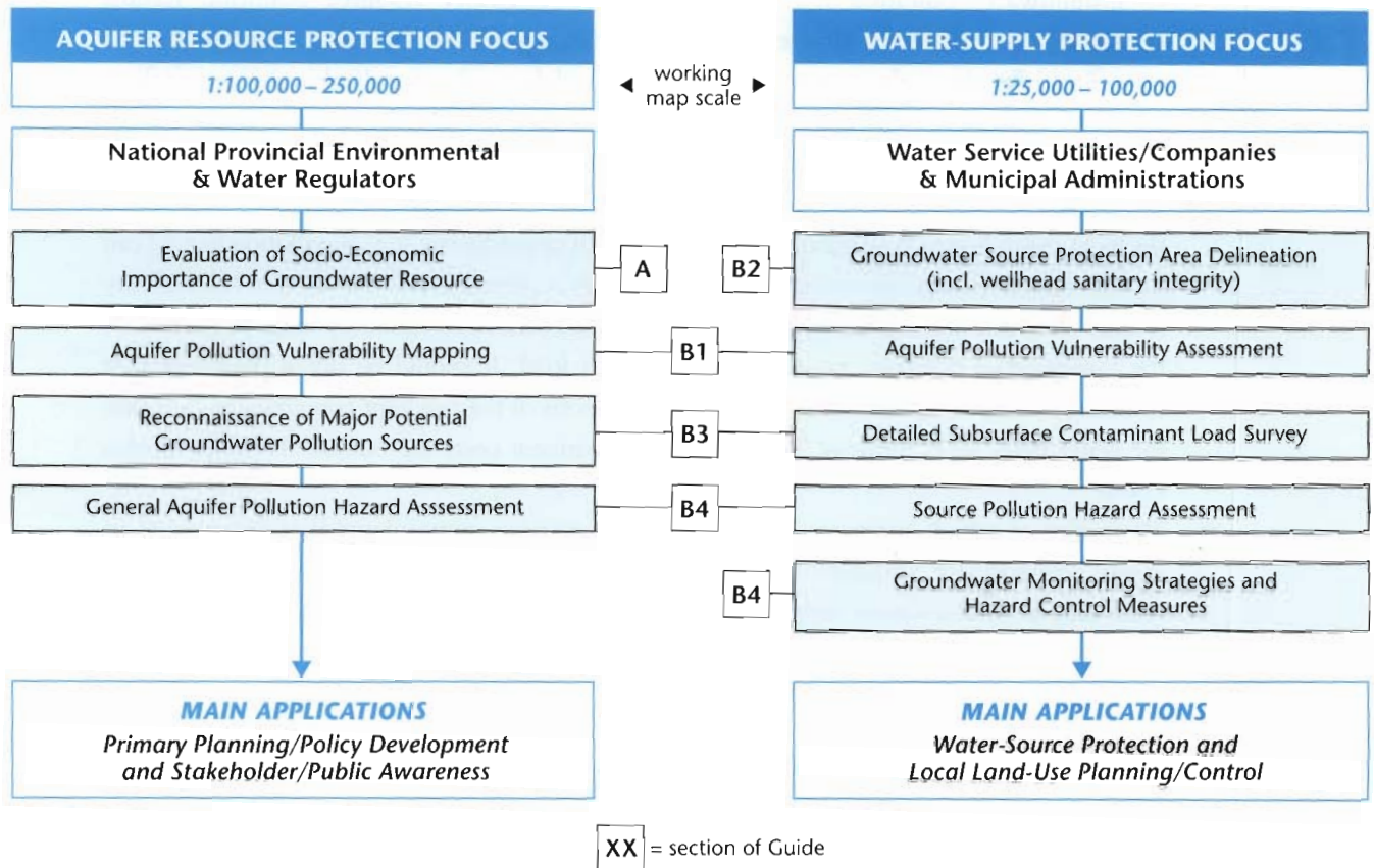
Figure A.4 Focus and application of different levels of groundwater pollution hazard assessment
