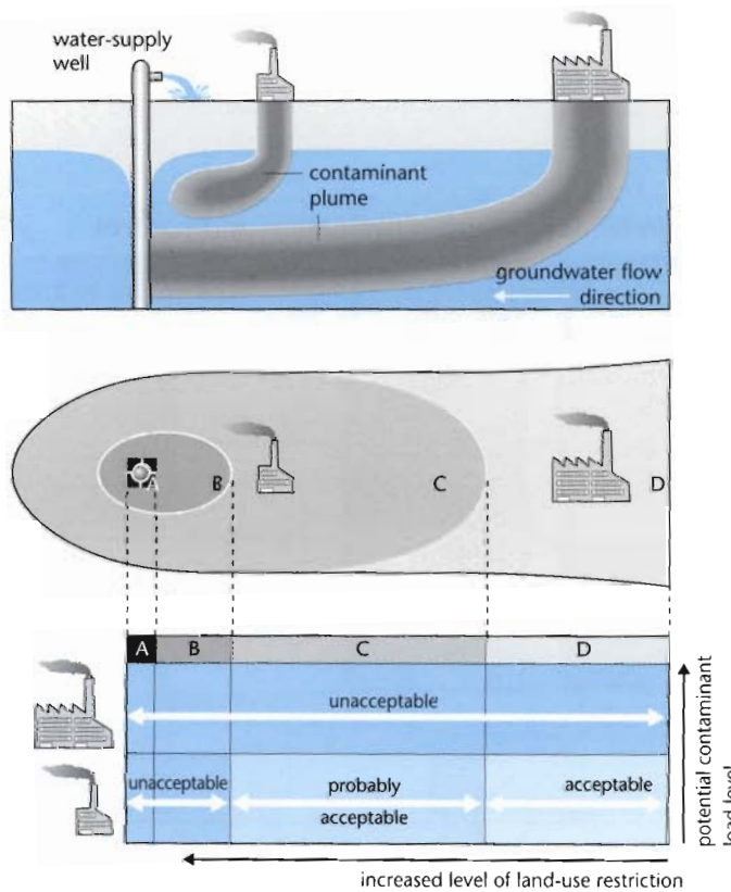
Figure A.5 Concept of groundwater source protection areas with land-use restrictions
