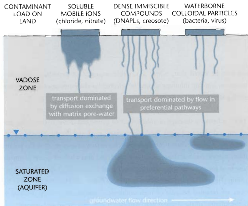
Figure 1.3 Development and consequences of preferential flow in the vadose zone
