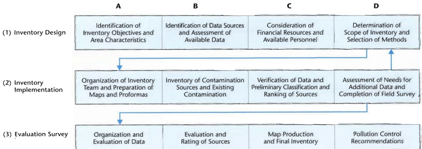
Figure 3.1 Development of an inventory of potential sources of subsurface contaminant load
