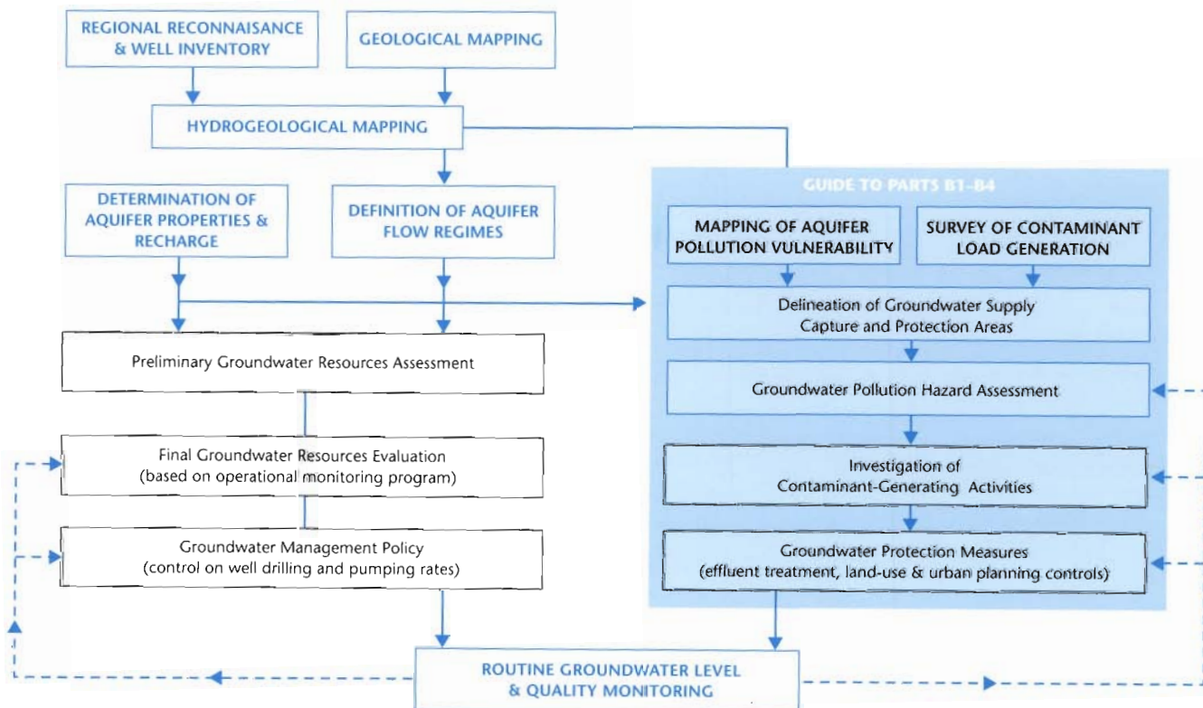
Figure A.7 Scope of Guide in context of overall scheme of groundwater resource management
