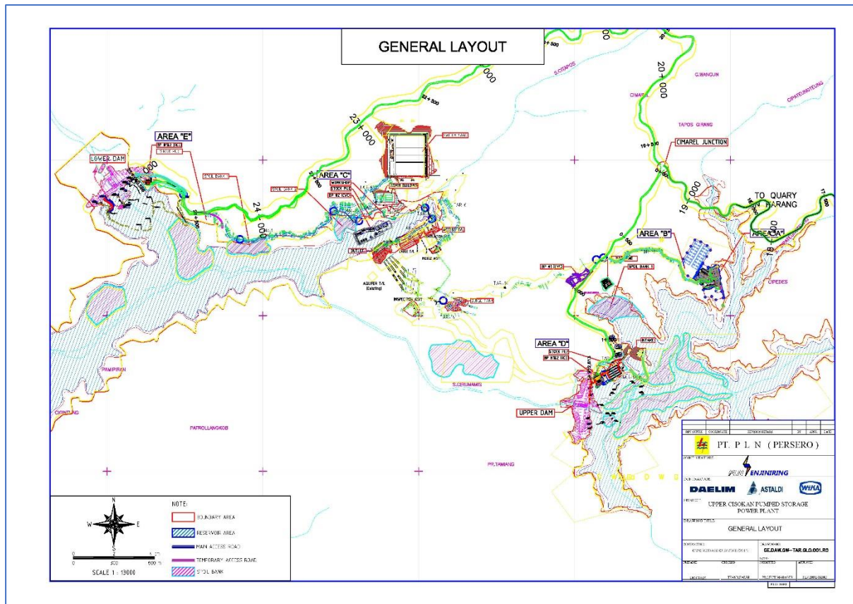
Gambar 2. Skema Tata Letak UCPS (Upper Cisokan Pumped Storage)
