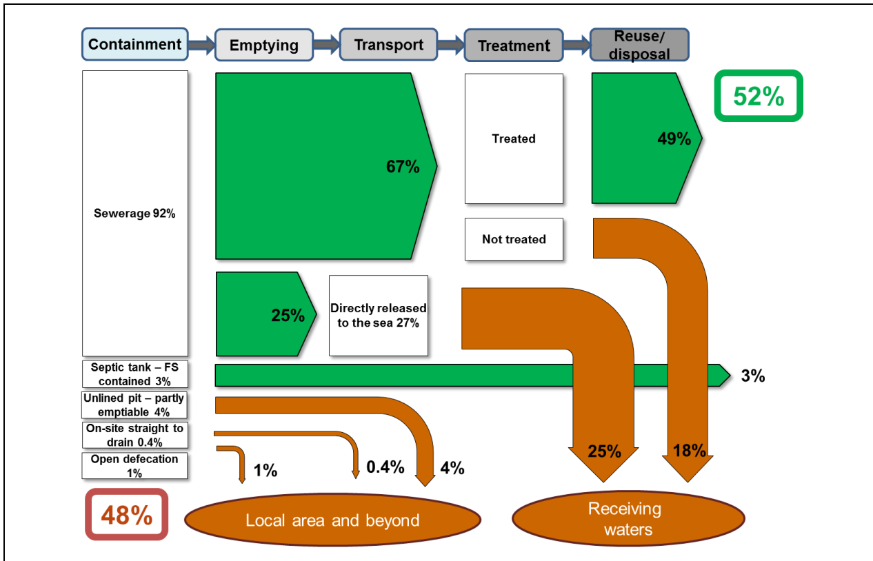
Figure 5 City-wide fecal waste flow diagram for Lima, Peru
