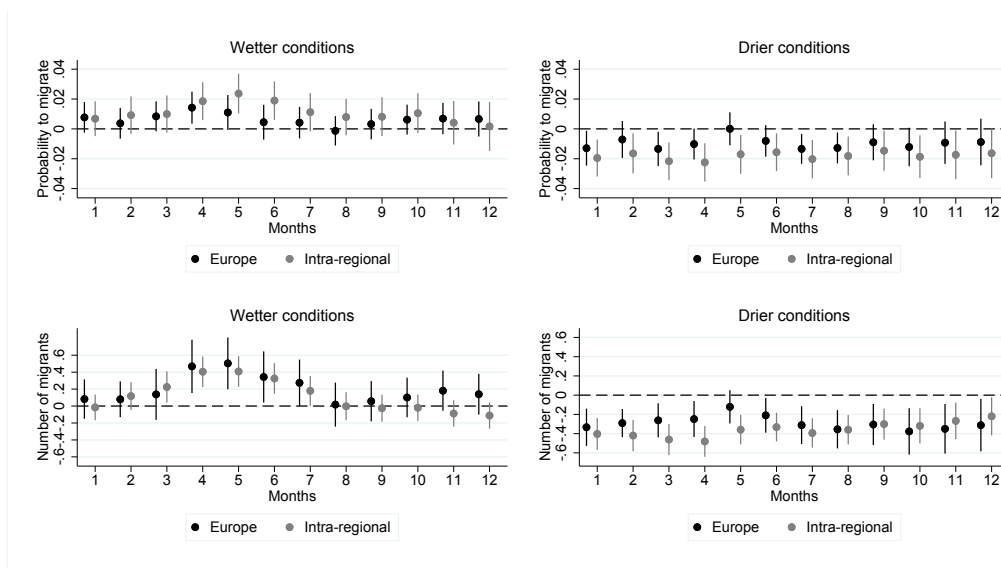
Figure 6: EFFECT OF POSITIVE AND NEGATIVE SOIL MOISTURE SHOCKS BY DESTINATION
