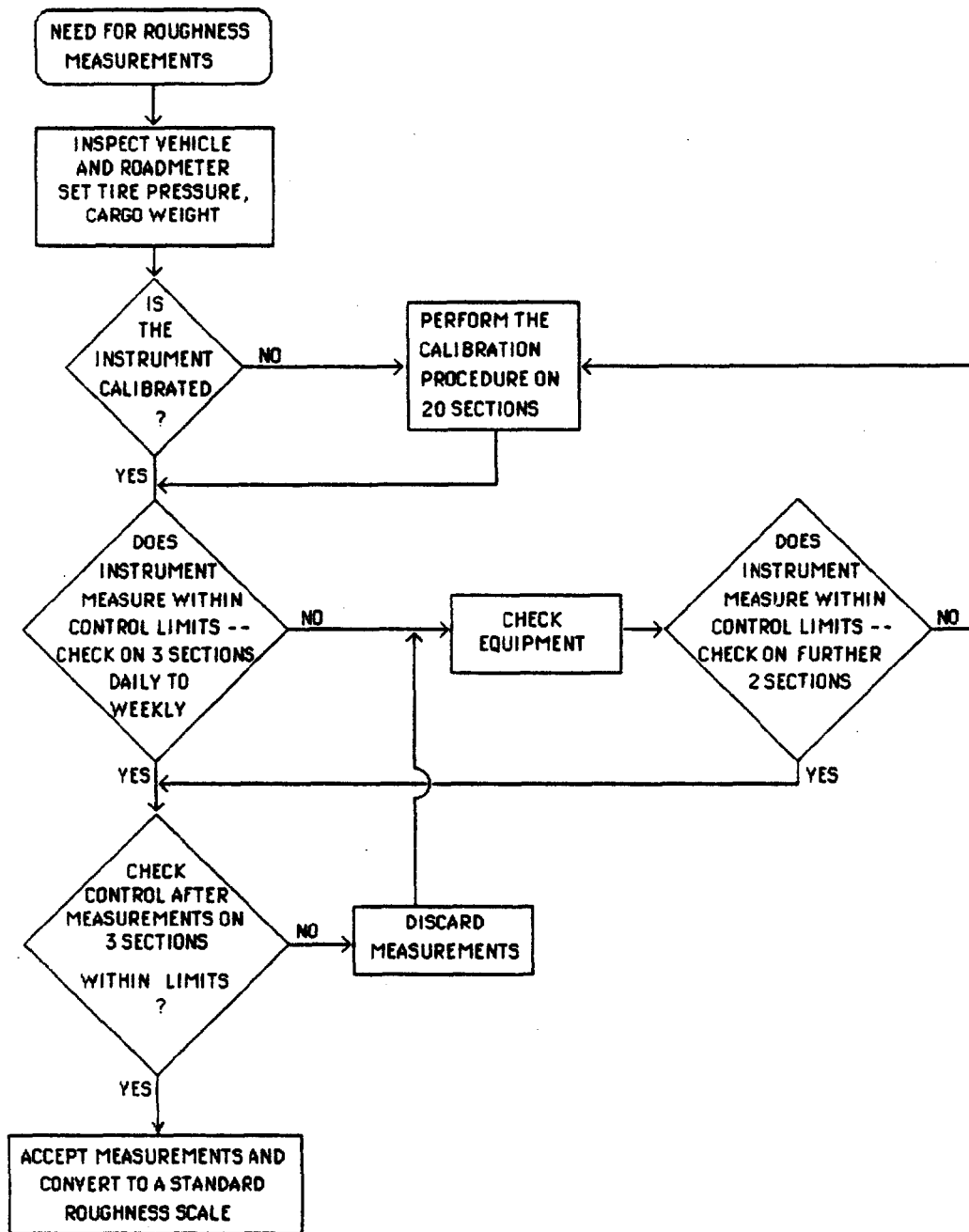
Fig. 8 Logic diagram for RTRRMS operation
