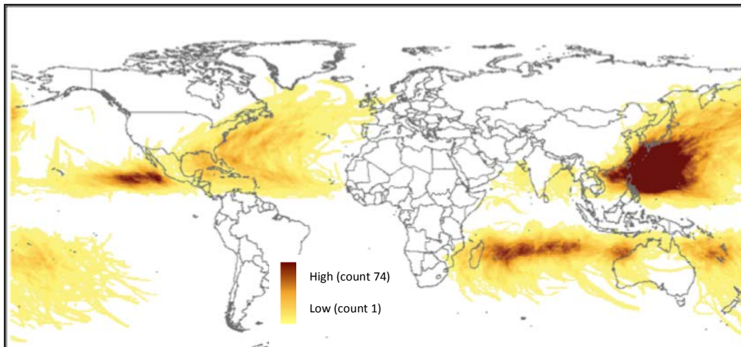
Figure 3: Global cyclone frequency 1975-2007
