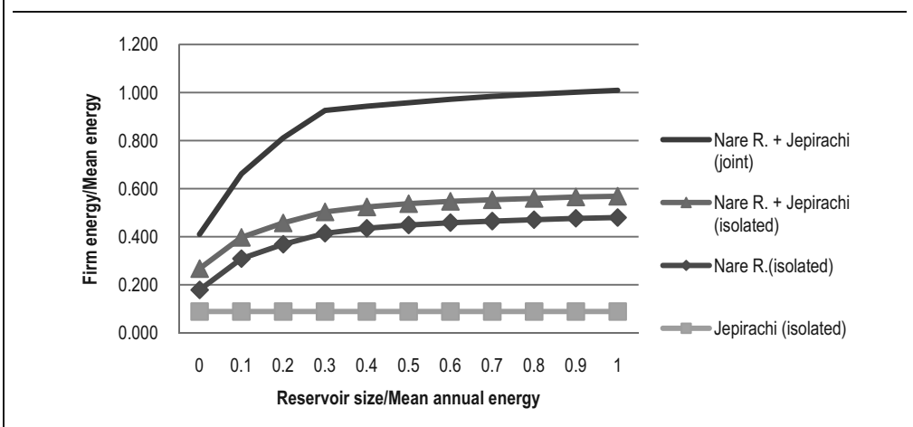
Figure A6.16. Firm Energy for Nare and Jepirachi in Isolated and Joint Operation
