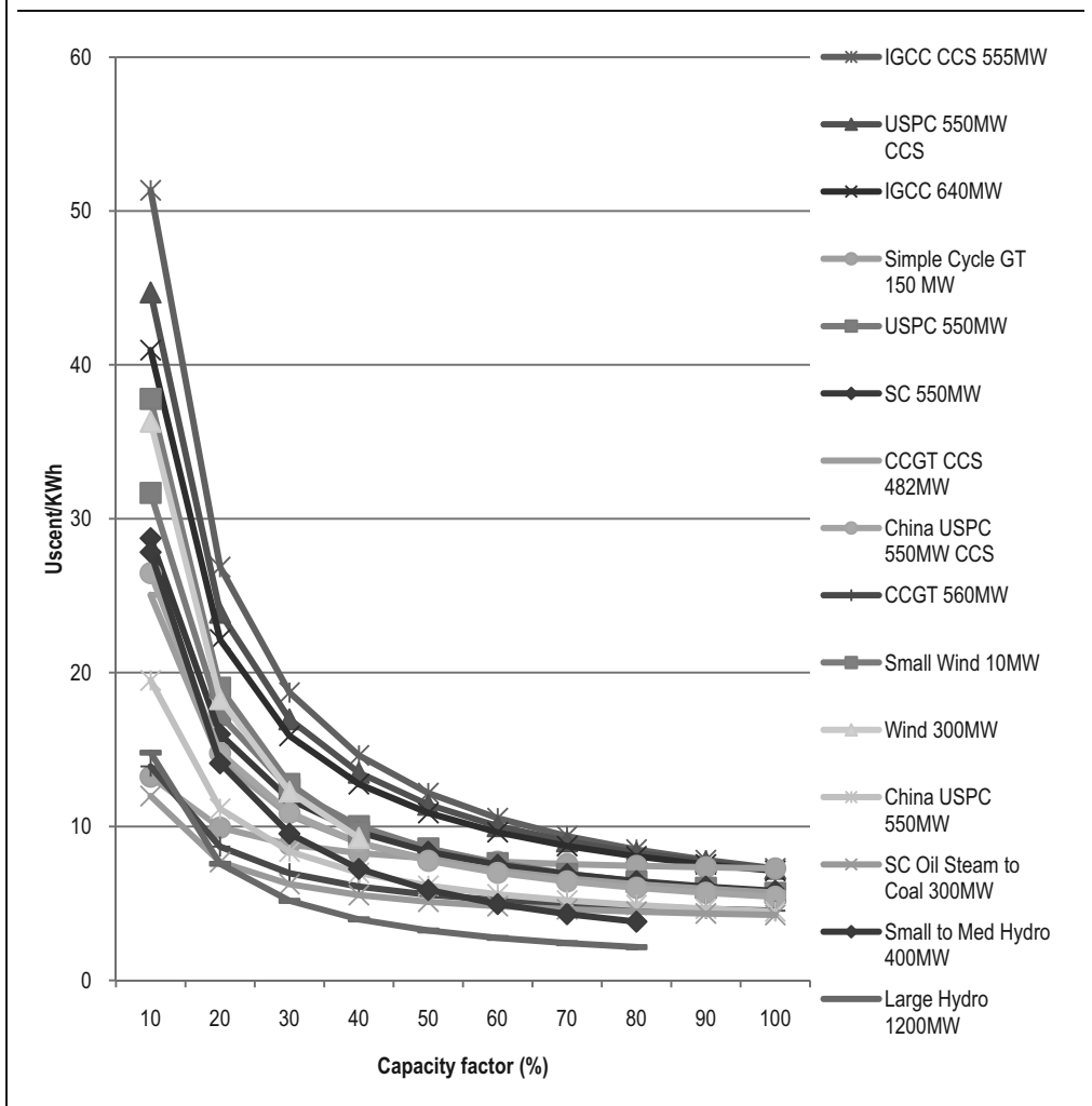
Figure 3.2. Screening Curve for Levelized Total Costs at Different Capacity Factors Measured in Terms of Generation Costs (US cents/kWh)
