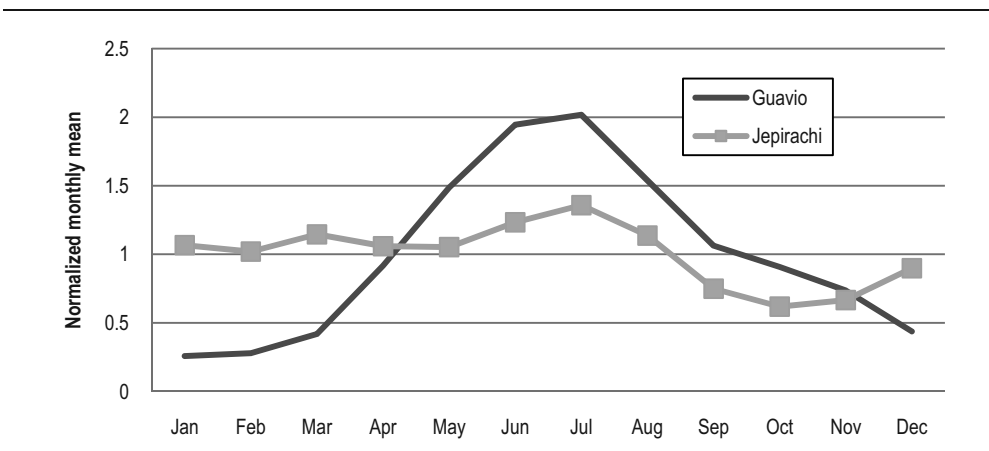
Figure A6.9. Mean Monthly Values at the Guavio River Dam Site
