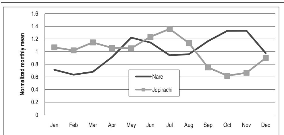
Figure A6.10. Mean Monthly Values at the Santa Rita Dam Site on the Nare River
