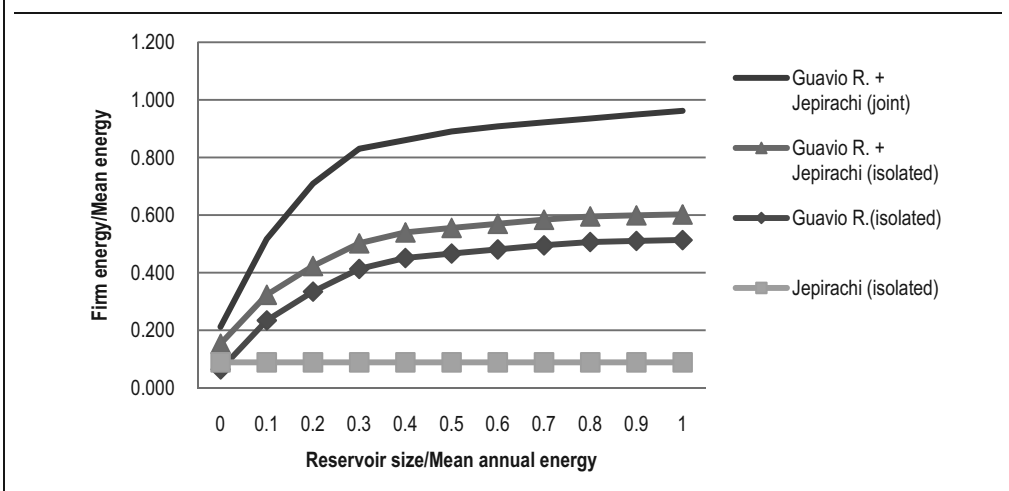
Figure A6.13. Firm Energy for Guavio and Jepirachi in Isolated and Joint Operation
