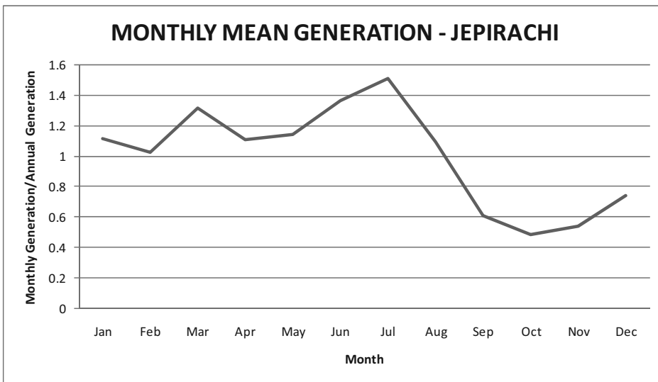
Figure A6.8. Jepirachi: Monthly Mean Generation
