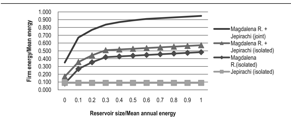
Figure A6.22. Firm Energy for Magdalena and Jepirachi in Isolated and Joint Operation
