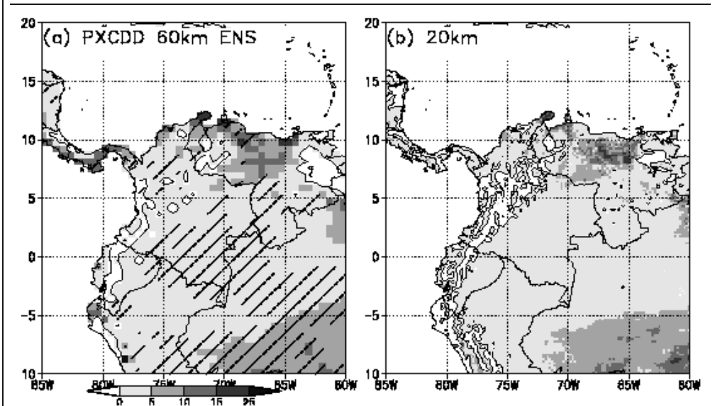
Figure A2.2. The Same as In Figure A.2.1 Except for Consecutive Dry Days (day)
