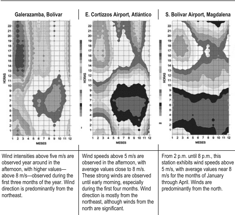
Figure 5.3. Graphic Representation of Wind Conditions in Northern Colombia
