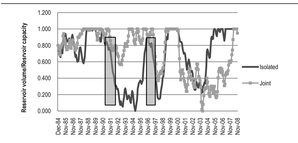
Figure A6.18. Nare River Reservoir Operation with Reservoir Size 0.5
