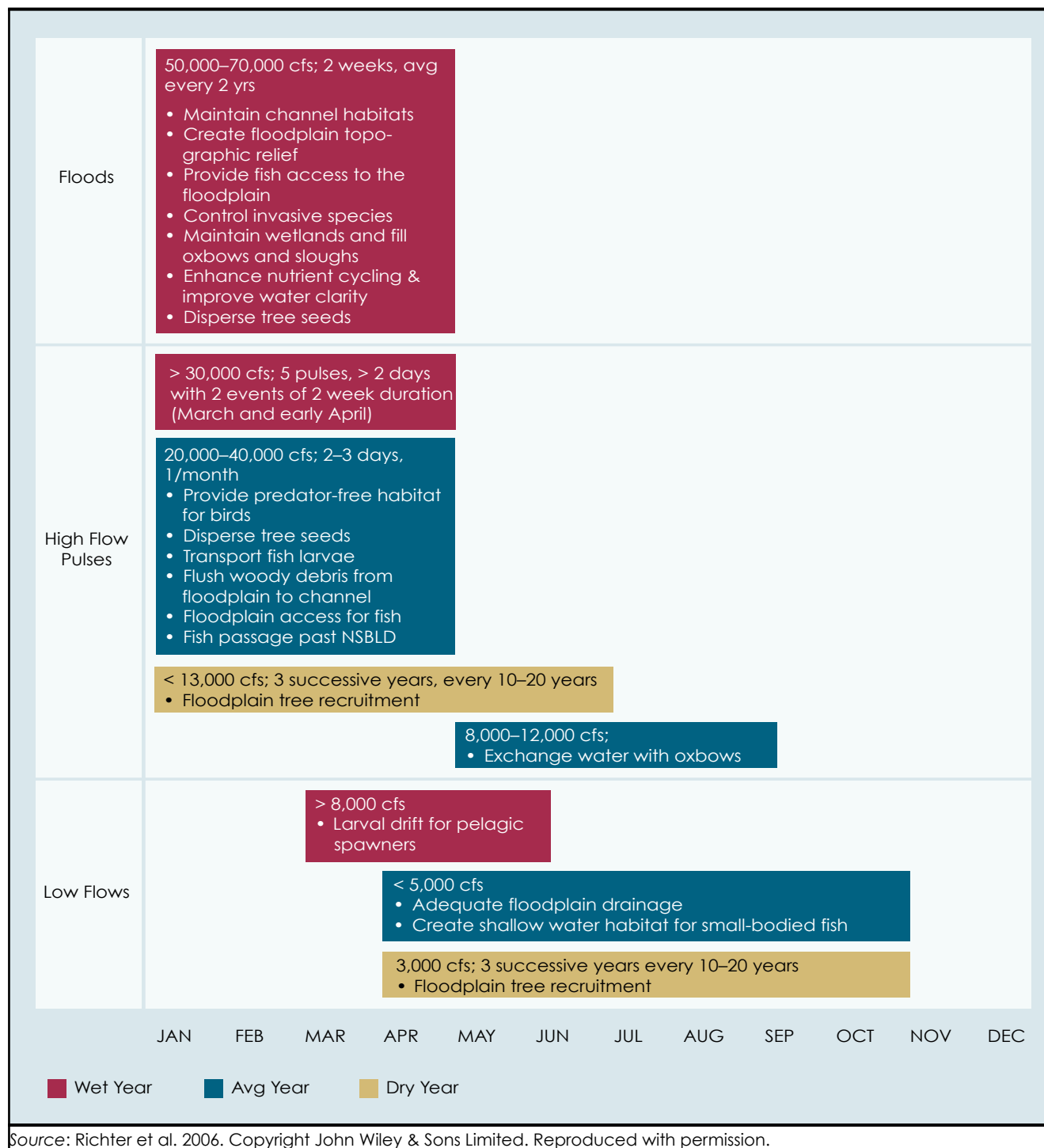
Figure 2. Environmental Flow Recommendations Developed for the Savannah River, U.S.
