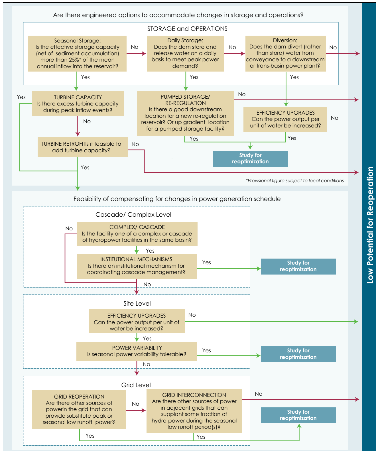
Figure 4. Screening Tool for Selecting Best Candidates for Dam Reoperation 1 (cont.)
