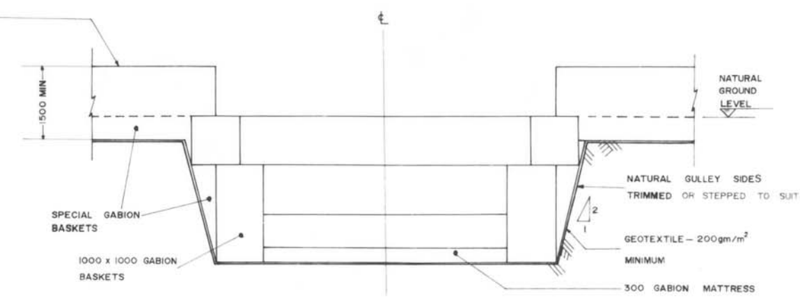
SECTION B-B
