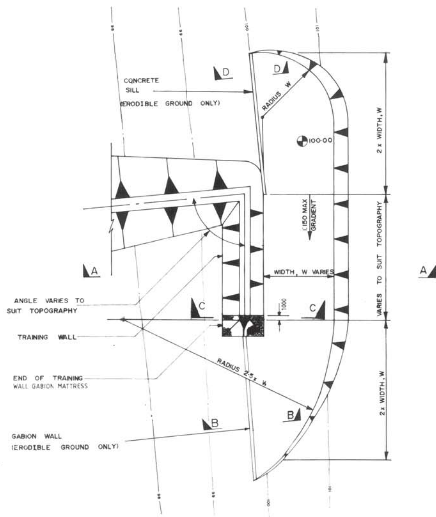
TYPICAL SPILLWAY ARRANGEMENT - PLAN
