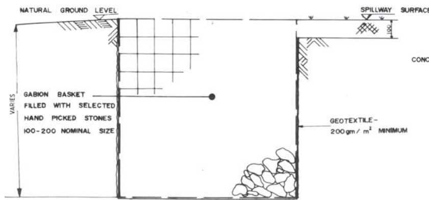
SECTION B-B - GABION WALL
