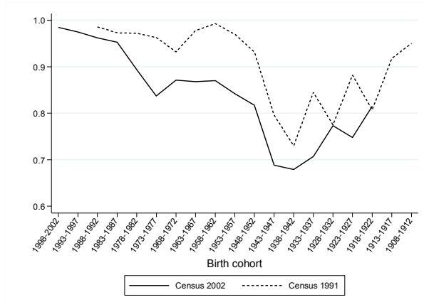
Fig. 1: Sex ratio by age group
