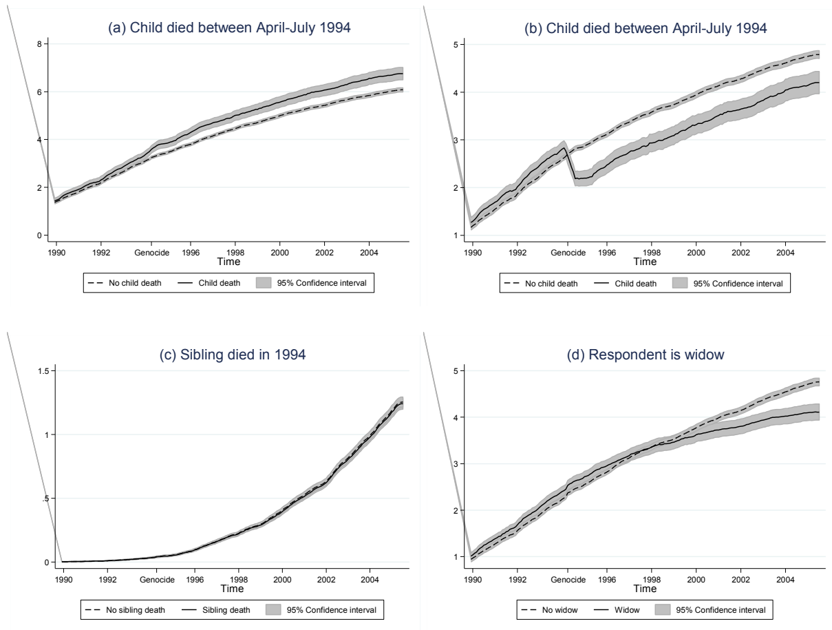
Fig. 5: Predicted fertility over time
