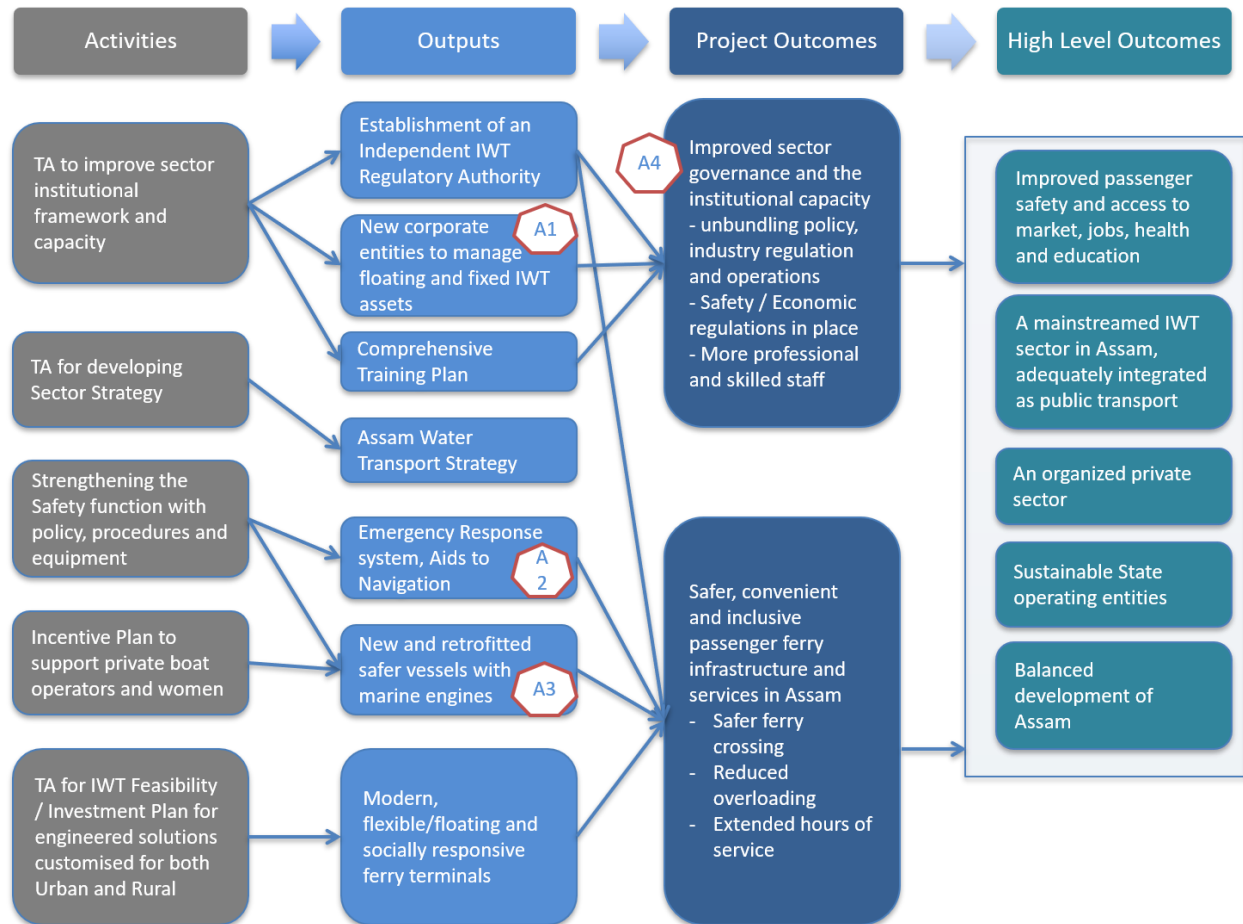
Figure 1. Results Chain
