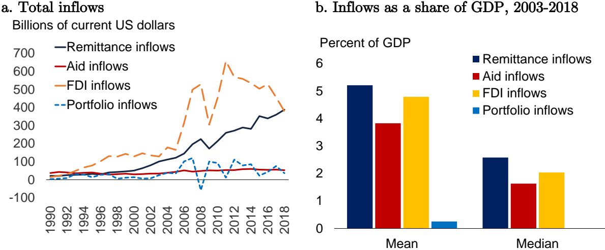
Figure 1. Remittances, aid and capital inflows to EMDEs
