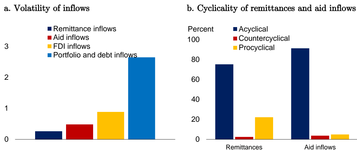
Figure 2. Cyclical properties of capital flows to EMDEs
