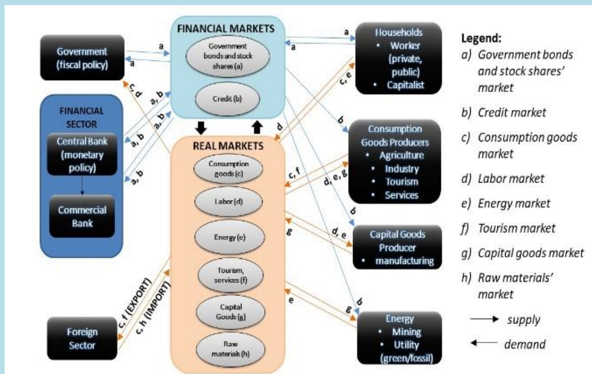
(a) Agents, sectors and markets of the EIRIN economic model.
