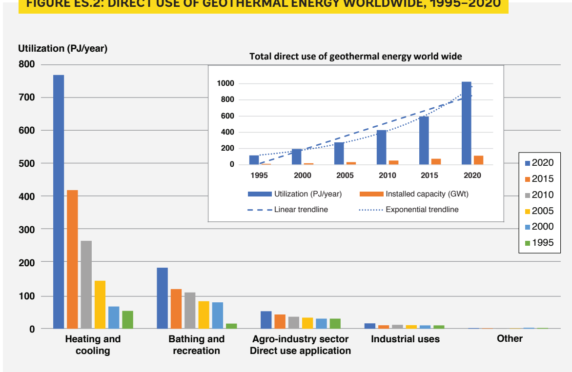
FIGURE ES.2: DIRECT USE OF GEOTHERMAL ENERGY WORLDWIDE, 1995–2020
