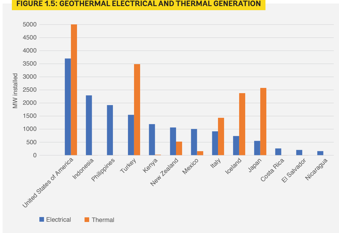
FIGURE 1.5: GEOTHERMAL ELECTRICAL AND THERMAL GENERATION
