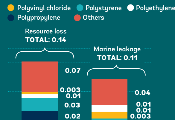
Figure 6: Contribution (million tons of plastic) of the fisheries sector to plastic waste and marine litter in 2021, by polymer and product
