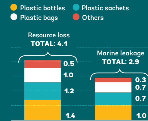
Figure 4: Contribution (million tons of plastic) of the packaging sector to plastic waste and marine litter in 2021, by polymer and product
