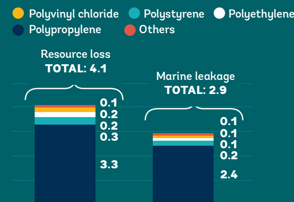
Figure 4: Contribution (million tons of plastic) of the packaging sector to plastic waste and marine litter in 2021, by polymer and product
