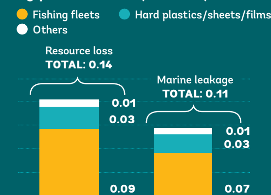
Figure 6: Contribution (million tons of plastic) of the fisheries sector to plastic waste and marine litter in 2021, by polymer and product
