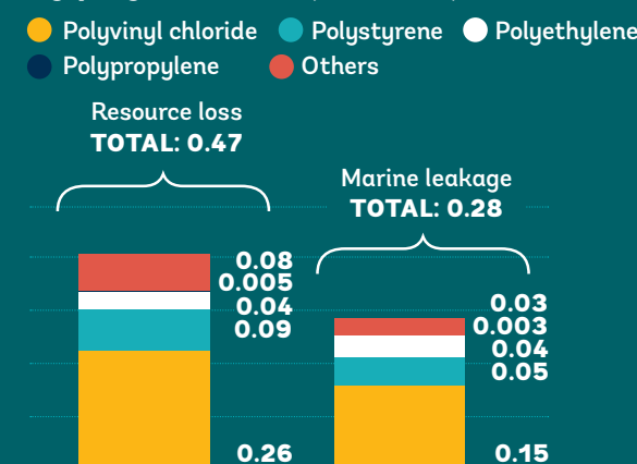
Figure 5: Contribution (million tons of plastic) of the construction sector to plastic waste and marine litter in 2021, by polymer and product
