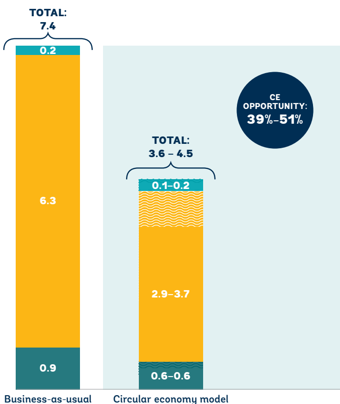
Figure 17: Plastic resource loss mitigation based on a pragmatic circular economy scenario in 2026 (million tons)
