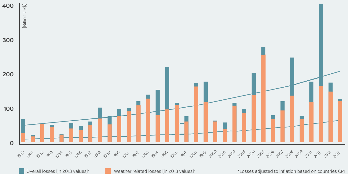
Figure 1: Disaster and weather-related losses 1980–2013
