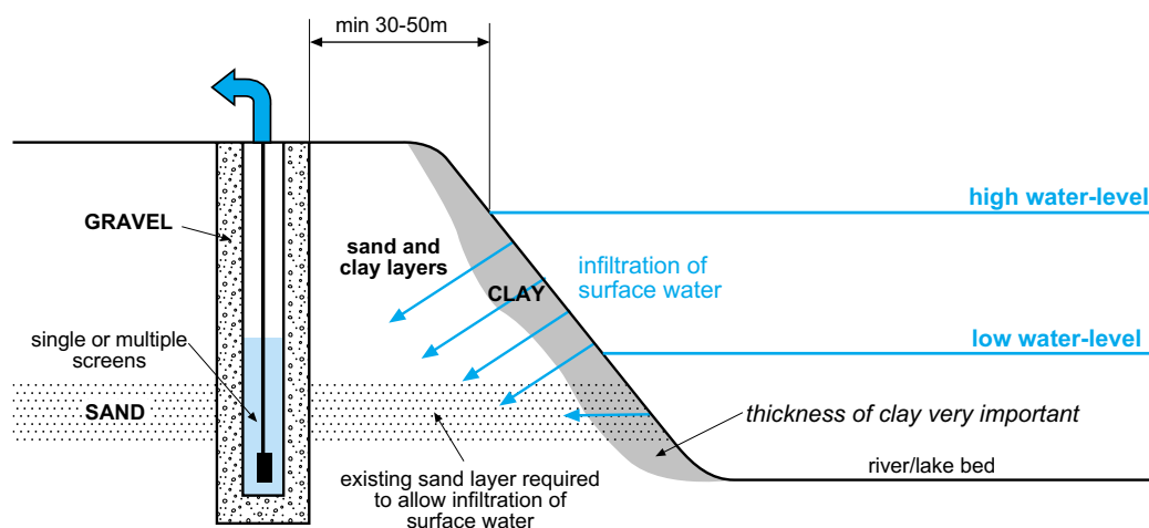
Figure 4 : Design of an induced surface-water infiltration scheme
