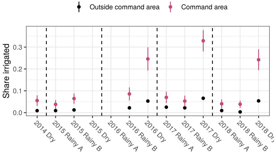
Figure 3: Adoption dynamics
