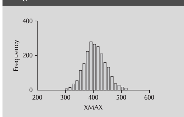
Figure 33 Simulated Distribution of the XMAX
