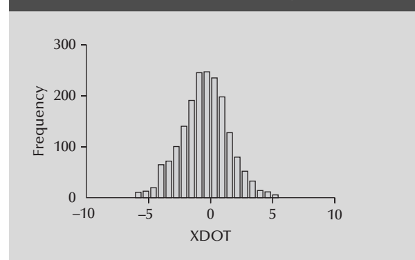
Figure 34 Simulated Distribution of Biomass Growth in Base Year, XDOT
