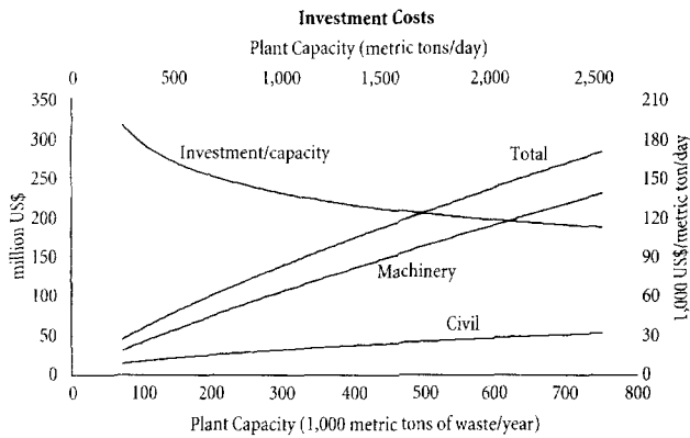
Figure 7 Estimated Cost of Incineration Plants
