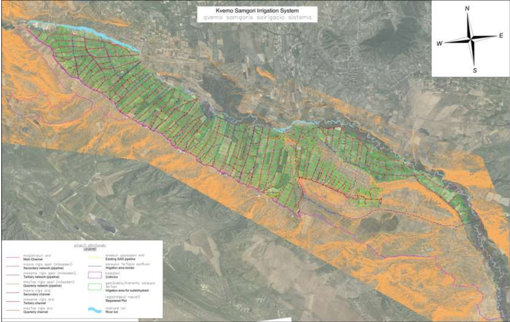
Figure 1: Project Layout
