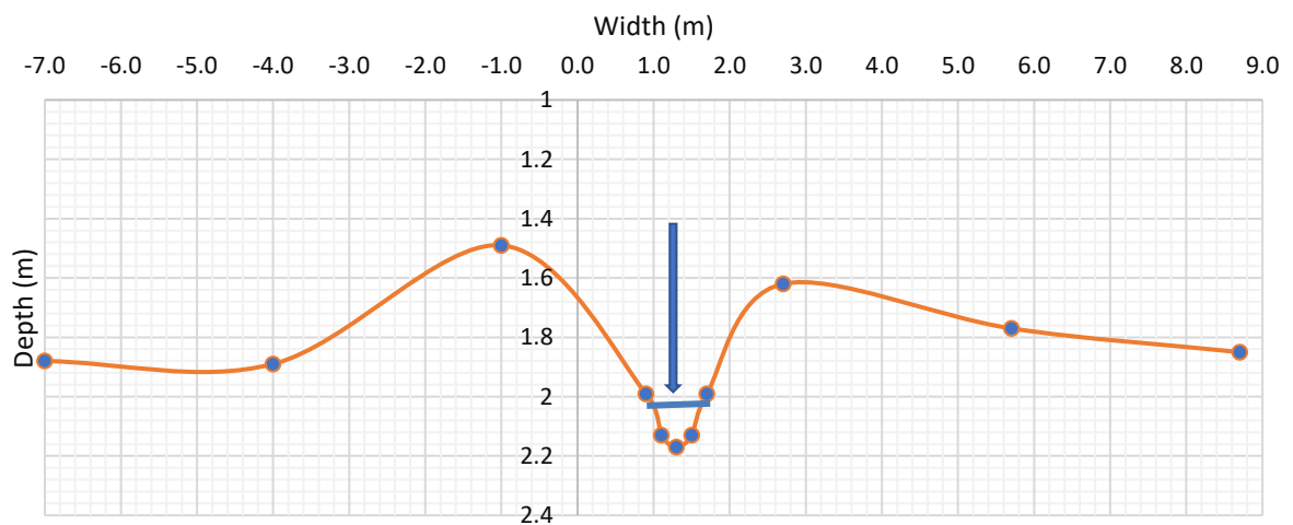
k) Cross Section at Point 12 - River Rwemango
