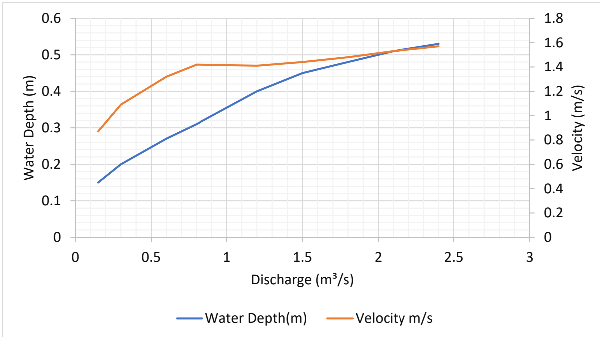
Figure 6-14: Discharge against water depth and velocity at sampling point 15
