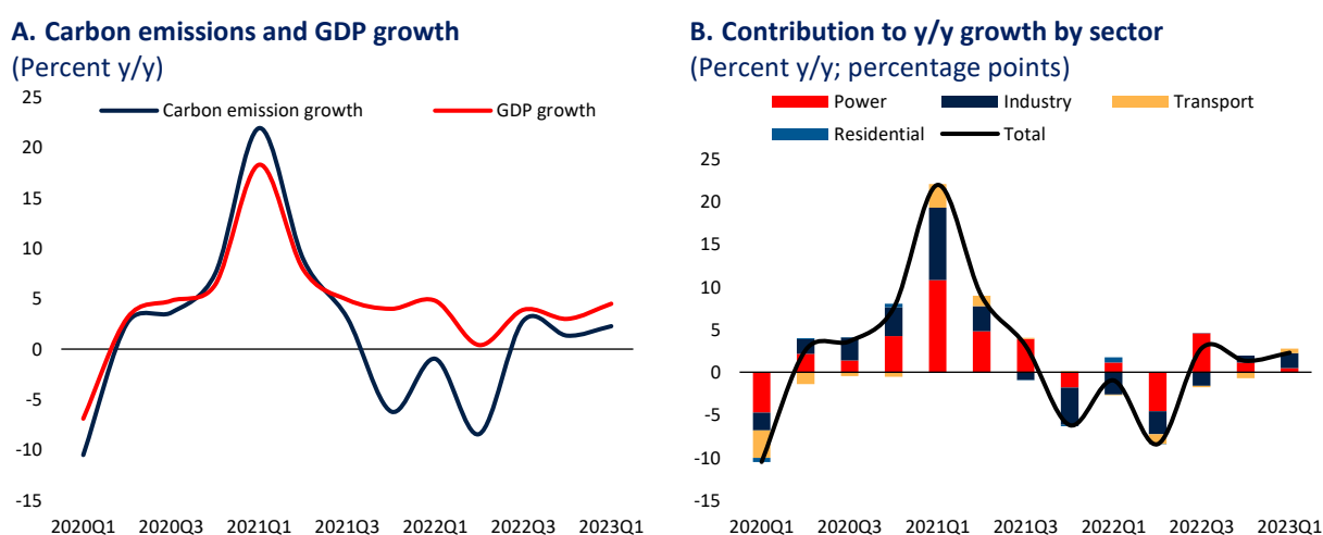
Figure 8. Carbon emissions grew moderately in the first quarter of 2023
